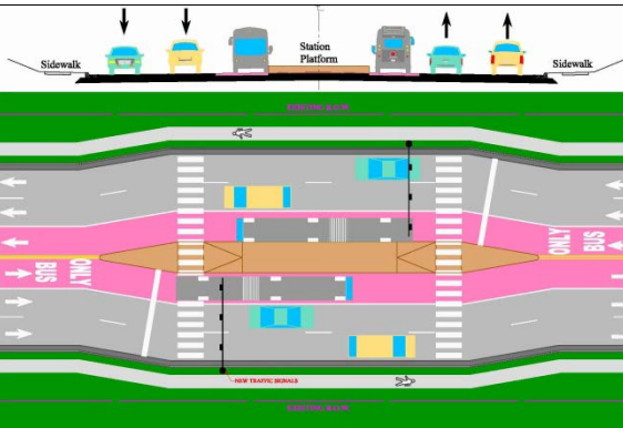
BRT in dedicated median lanes at median station
