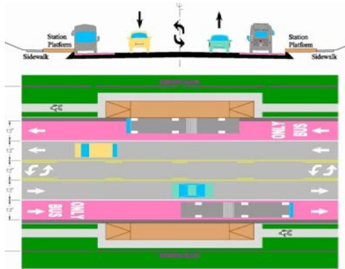
BRT in dedicated outside lanes at side stations
