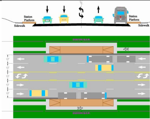
BRT in mixed traffic at side stations
